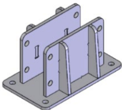
Side Mount '95mm offset' Chassis Mount (only suitable for 150mm RHS Chassis)
