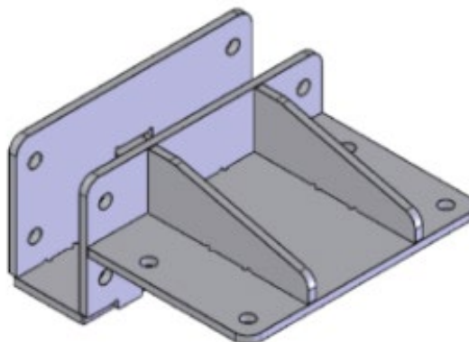
Side Mount '95mm offset' Chassis Mount (only suitable for 150mm RHS Chassis)
