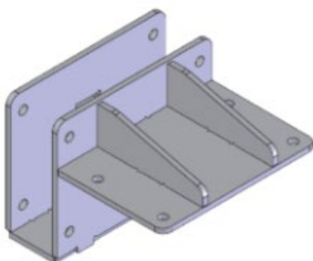
Side Mount '95mm offset' Chassis Mount (only suitable for 150mm RHS Chassis)
